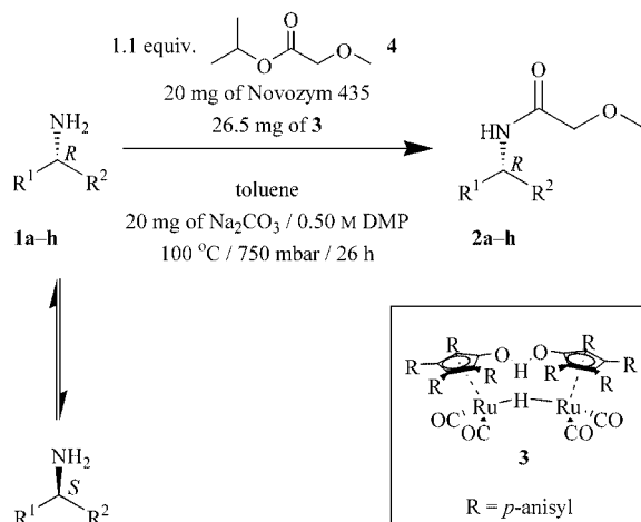
Scheme 1. DKR of amine substrates 1a–h (DMP: 2,4-dimethyl-3-pentanol, added as hydrogen donor).
